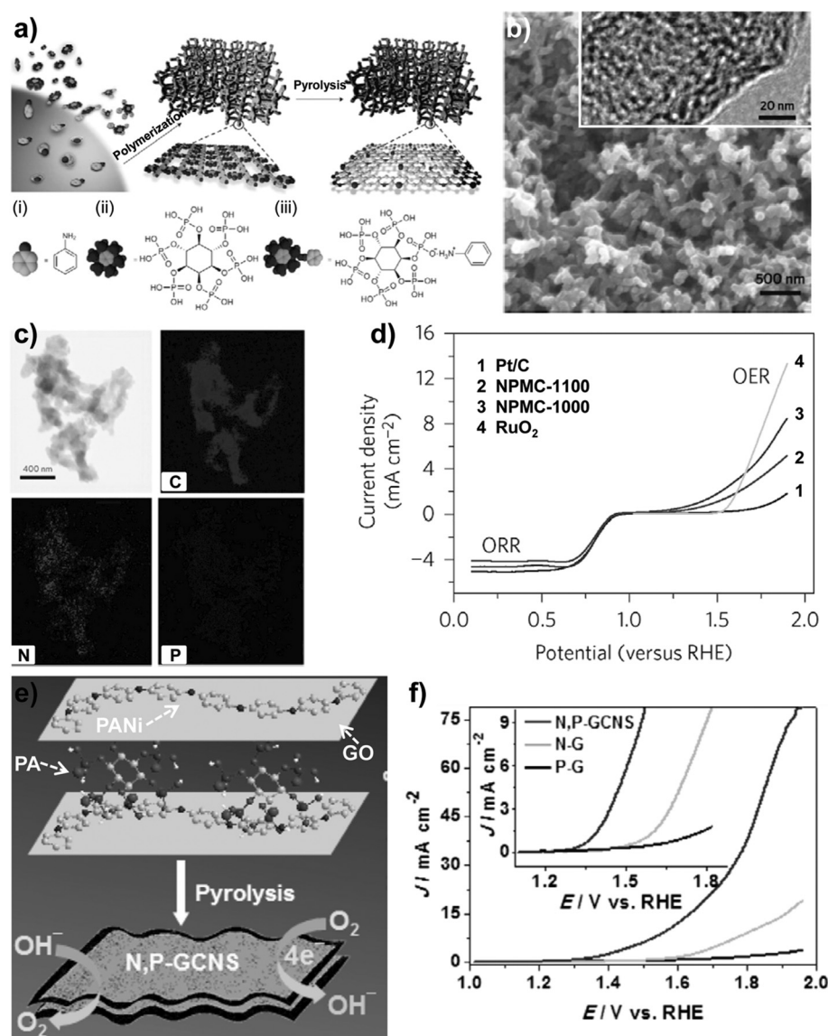
Figure 4. a) Schematic illustration of the preparation of the NPMC foams. Aniline (i) and phytic acid (ii) form a complex (iii), which undergoes oxidative polymerization into a 3D PANi hydrogel network. The PANi hydrogel is then freeze-dried and pyrolyzed in Ar to produce the NPMC. b) SEM image of NPMC-1000. Inset: the high-resolution TEM image. c) TEM image and corresponding element mapping images of NPMC-1000. d) LSV curves of NPMC-1000, NPMC-1100, RuO 2 , and the commercial Pt/C catalyst on an RDE in 0.1 M KOH solution, showing the electrocatalytic activities for both the ORR and OER (reprinted from Ref. [81] with permission. Copyright 2015 Nature Publishing Group). e) Schematic illustration of the fabrication process and structure of the N- and P-doped bifunctional GCNS oxygen electrocatalyst. f) Comparison of the OER activity of various catalysts in 0.1 M KOH solution evaluated by LSV tests. Inset: Magnified view (reprinted from Ref. [82] with permission. Copyright 2015 American Chemical Society).
